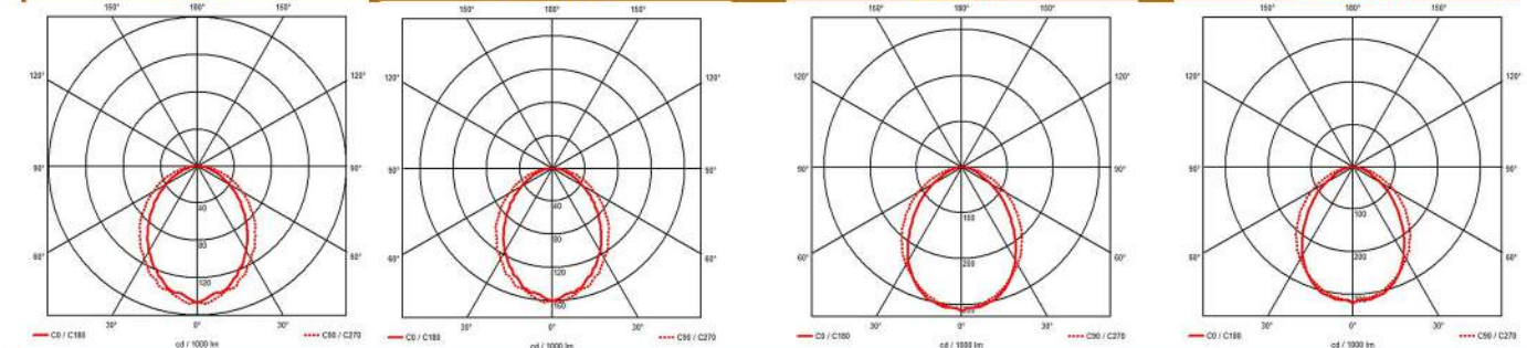
Atlas 1 Prismatic Reflector 2x14W Atlas 1 Prismatic Reflector 2x21W Atlas 1 Prismatic Reflector 2x24W Atlas 1 Prismatic Reflector 2x28W
