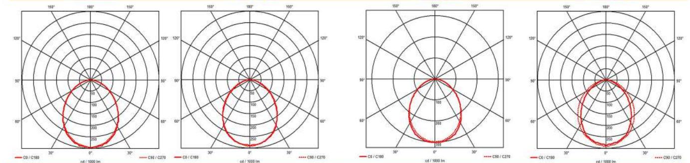
Atlas 1 Prismatic Reflector 2x35W Atlas 1 Prismatic Reflector 2x39W Atlas 1 Prismatic Reflector 2x54W Atlas 1 Prismatic Reflector 2x80W
