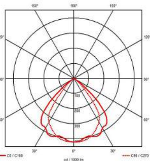
Atlas 1 Louver 2x54W
