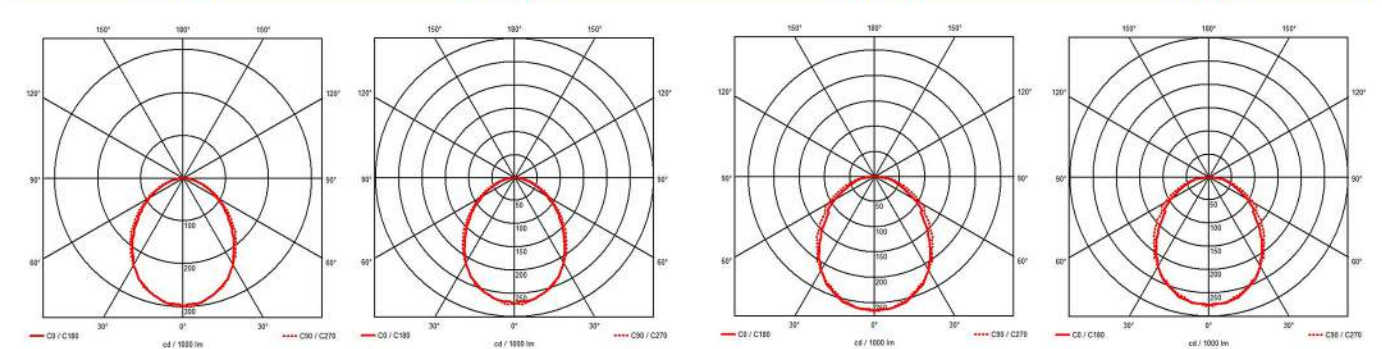
Atlas 1 Prismatic Reflector 2x35W Atlas 1 Prismatic Reflector 2x39W Atlas 1 Prismatic Reflector 2x54W Atlas 1 Prismatic Reflector 2x80W
