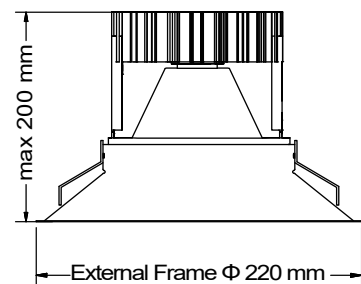
Cutting Hole Diameter 200 mm
