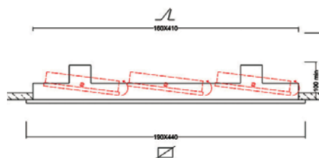
Cutting Hole 160 mm x 410 mm
