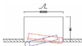
Cutting Hole 85 mm x 85 mm
