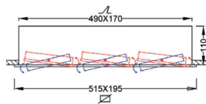
Cutting Hole 490 mm x 170 mm
